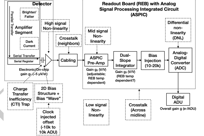
Figure 4. The model of the detector and Readout Electronics Board (REB) components, labeled with the effects that they impart on signal.
