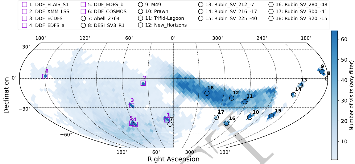
Figure 3. Sky distribution of DP2 visits across the three components of the observing program. Small-field survey areas are marked with black circles and Deep Drilling Fields (DDFs) with violet squares. The SV wide survey covers \sim 3,000 \text{ deg}^2 tracing the ecliptic plane, with visit density increasing toward the \sim 300 \text{ deg}^2 core. Pre-LSST Early Operations observations appear as sparser, predominantly i -band coverage extending across a larger area of the LSST footprint.
