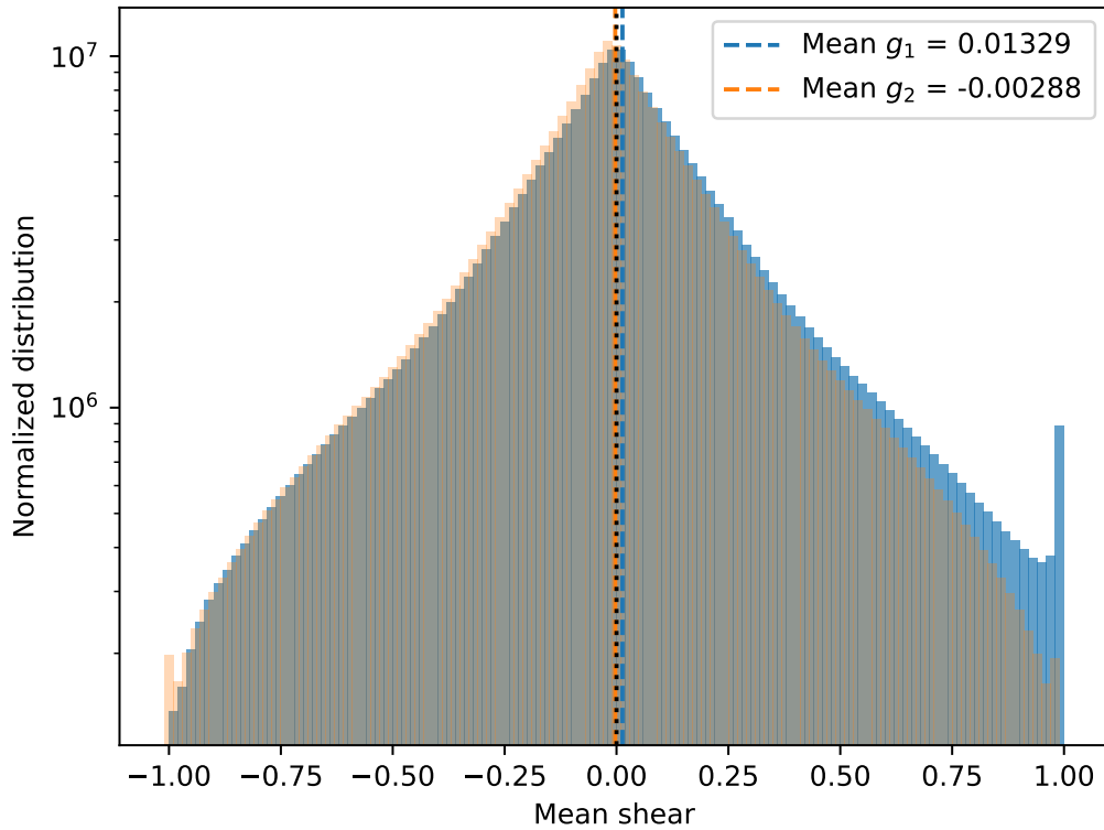
Figure 6. Distribution of gauss_g1 and gauss_g2 values for the ShearObject catalog’s no-shear subcatalog. The mean values of g_1 and g_2 are marked as vertical lines.
