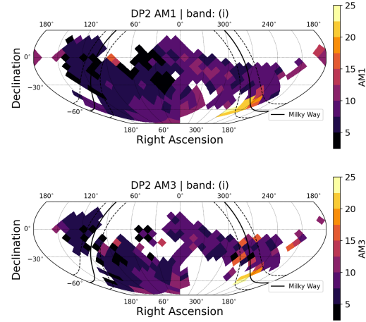
Figure 5. Median repeatability across all DP2 i-band visits for objects at 5 arcmin (top panel) and 200 arcmin (bottom panel). The difference in sky coverage is due to the fact that some regions of the sky do not have a sufficient number of objects separated by 200 arcmin.
