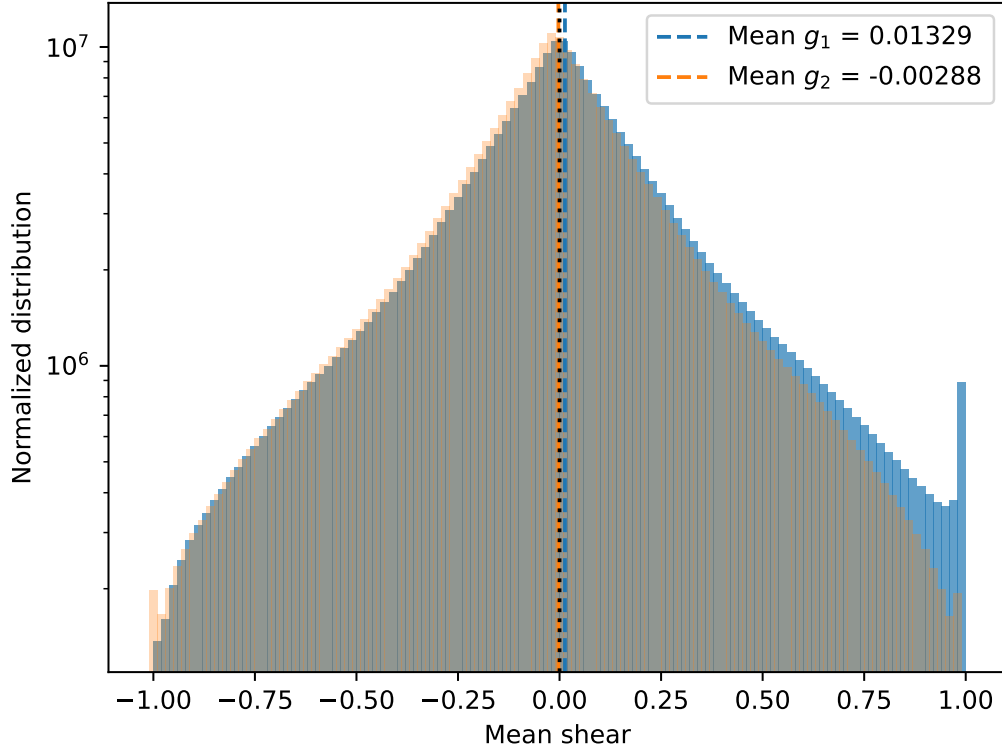
Figure 5. Distribution of gauss_g1 and gauss_g2 values for the ShearObject catalog’s no-shear subcatalog. The mean values of g_1 and g_2 are marked as vertical lines.
